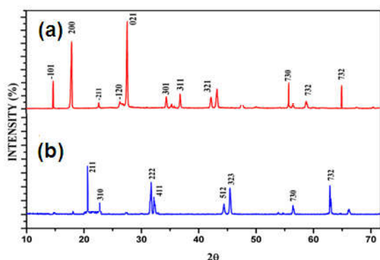
Fig 5 The XRD pattern of struvite obtained from Alpinia galanga root in the gel method (a) without any additive (b) with the 1.00% of methanol extract.
