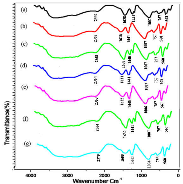
Fig 4 The FTIR spectra of struvite obtained from Alpinia galanga root in the gel method (a) without any additive (b) with the distilled water (c) with the 0.15% of methanol extract (d) with the 0.25% of methanol extract (e) with the 0.50% of methanol extract (f) with the 0.75% of methanol extract (g) with the 1.00% of methanol extract.
