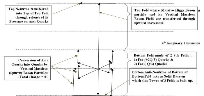
Fig. 11 Creation of Top Fold above Bottom Fold and Conversion of L.H. Anti Quarks into Quarks
