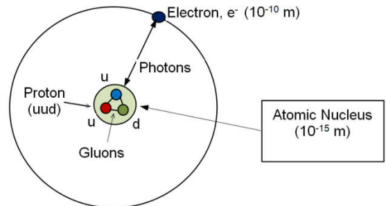
Fig 4 Hydrogen Atom
