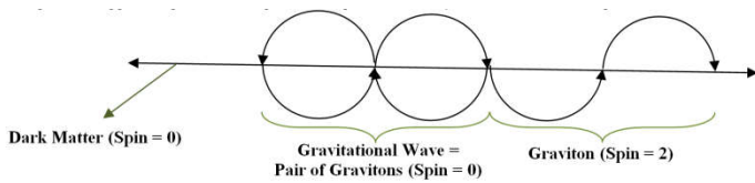
Fig 13 Gravitational Waves (Spin=0) made of Pair of Gravitons (Spin= ±2)
