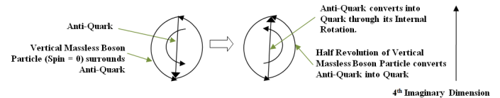
Fig 12 Conversion of Anti-Quarks (Anti-Matter) into Quarks (Matter)
