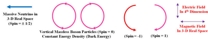
Fig 17 Nature of Neutrinos and Vertical Massless Bosons Particles
