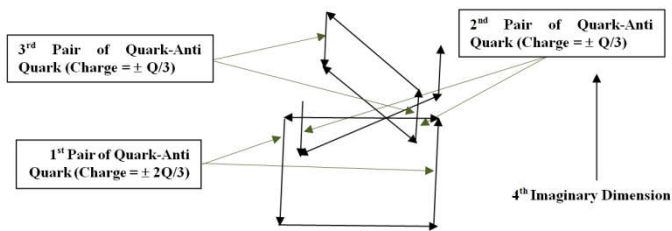
Fig 10 Creation of 3 rd Dimension and 3 Pairs of Quark-Anti Quark
