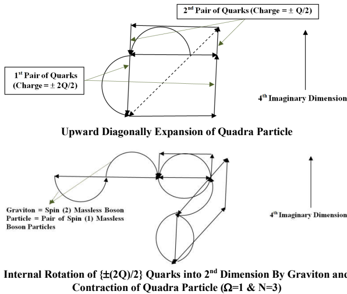
Fig 9 Creation of 2 nd Dimension and 2 Pairs of Quark-Anti Quark
