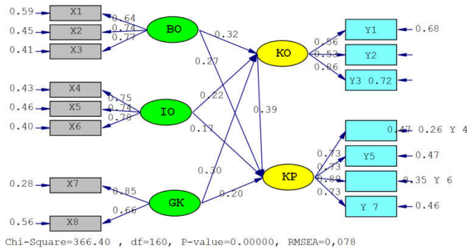
Figure 1 The Basic Model SEM (Standardized Model)
