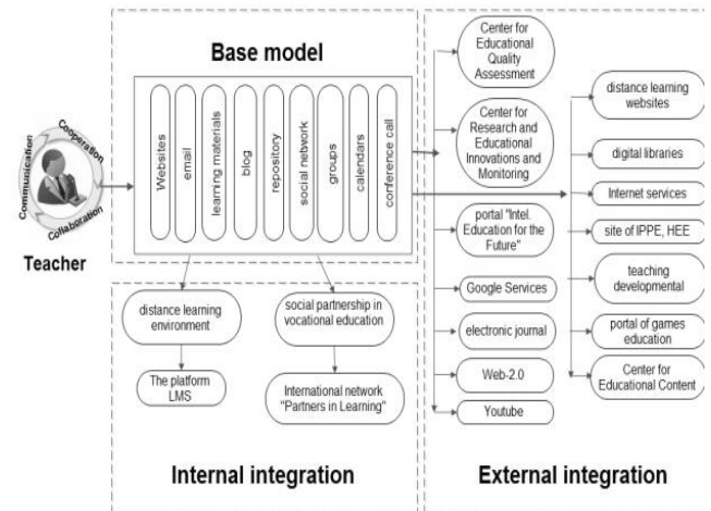
Figure 2 Integration of services in the basic model COLE of teacher
