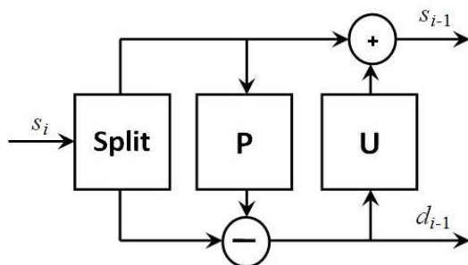
Figure2 Forward Lifting Scheme
